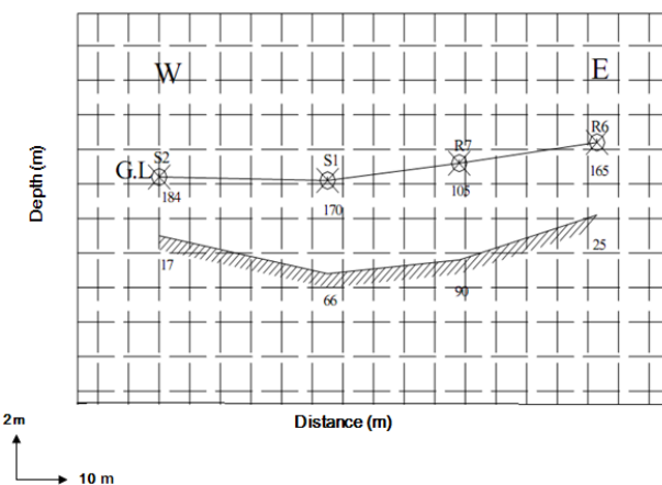
Figure 4) Geoelectric cross-section E.
