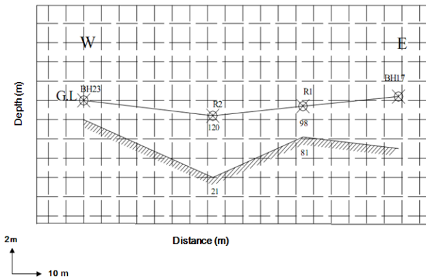
Figure 3) Geoelectric cross-section D.
