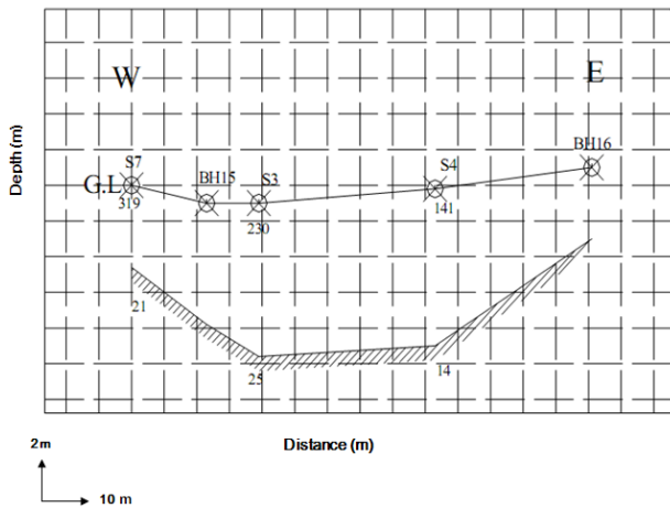
Figure 2) Geoelectric cross-section C.
