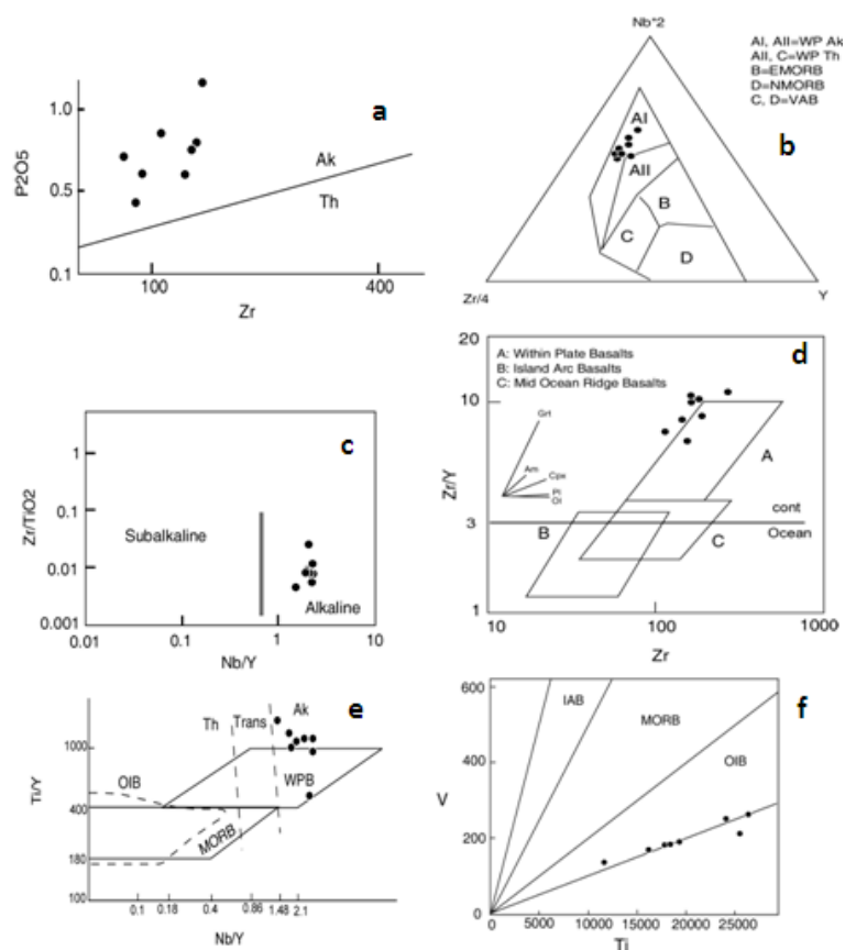
Figure 4) Various discriminations show that the MBG is alkaline within plate gabbro. a) Winchester and Floyd (1976), b) Meschede (1986), c) Vasquez and Althenberger (2005), d) Pearce (1983), e) Pearce (1982), f) Shervais (1982).
