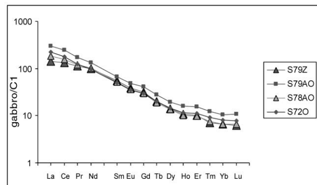
Figure 3) REE concentrations of MBG relative to Chondrite values from (Sun and McDonough, 1989).
