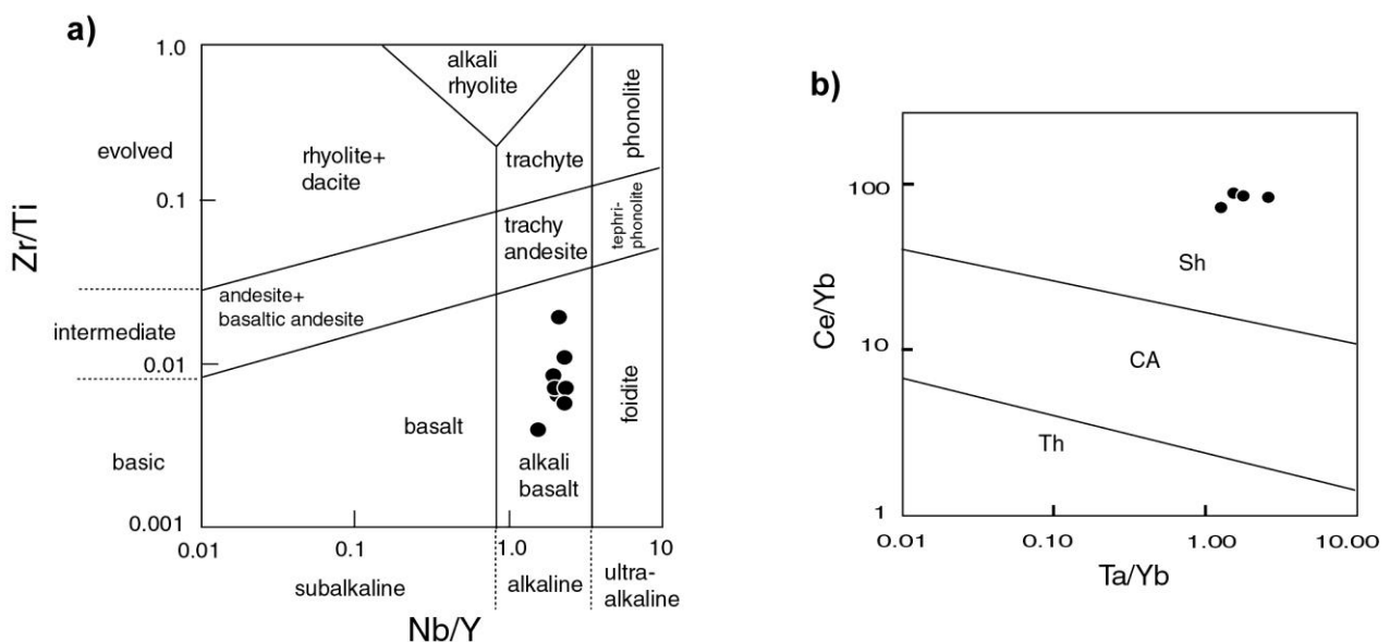
Figure 2a) Igneous rocks classifications after Middlemost (1995). All samples are alkali basalts. b) Shoshonitic affinity of MBG samples at the Muller and Groves (1993) diagram.
