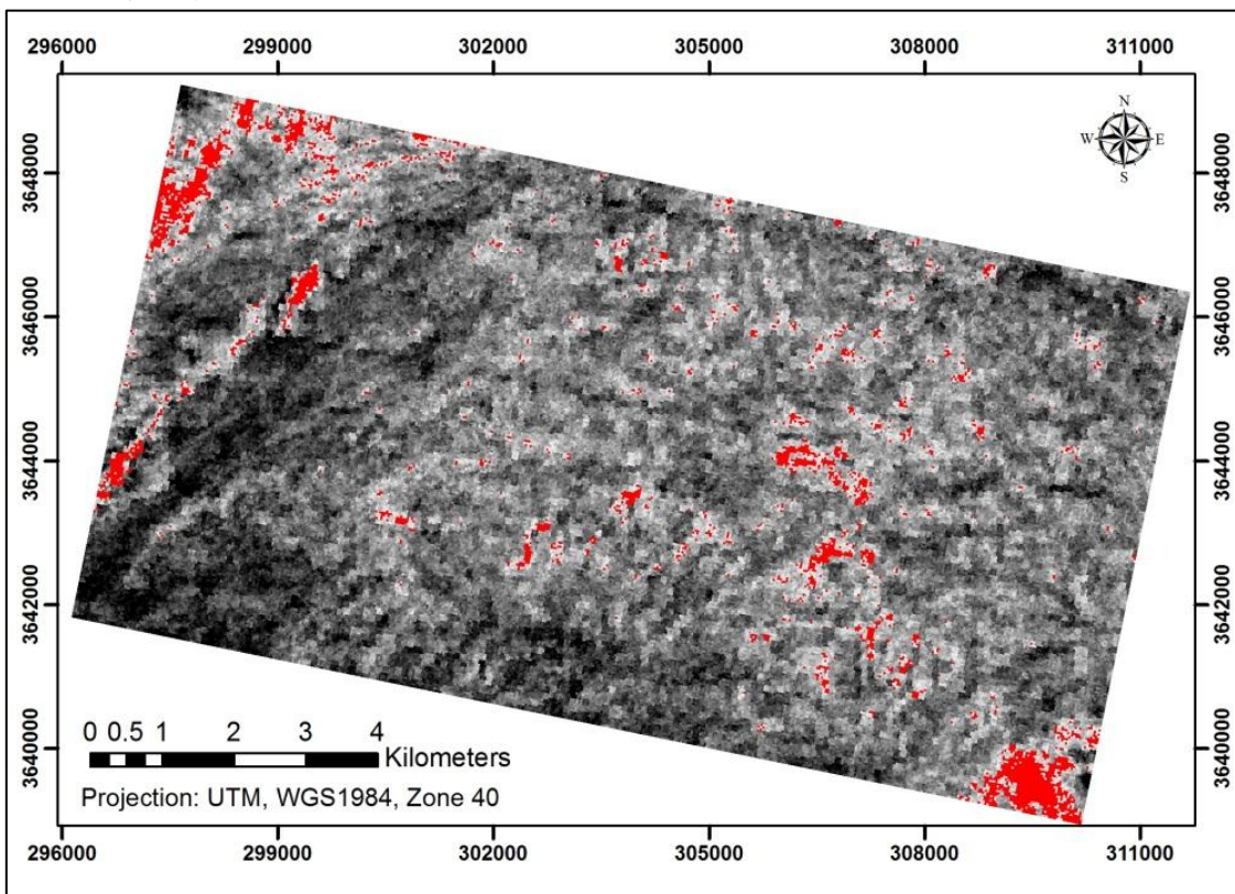
Figure 7) MF rule image of Quartz end member to indicate the silica-rich zones. Red pixels refer to the threshold of x+2s applied on the scene.
