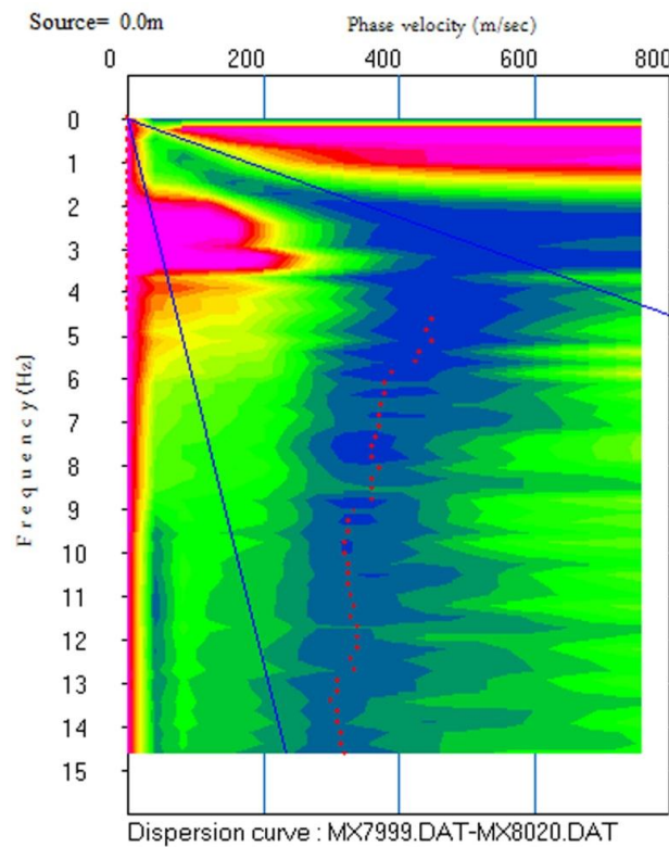
Figure 5) experimental dataset: a) a record of ReMi data, b) Dispersion curve.
