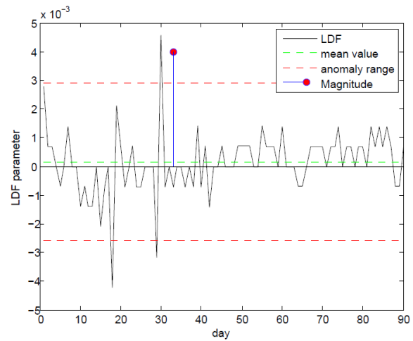
Figure 7) LDF parameter of Kashmar earthquake (from 1/1/2000 to 31/3/2000).
