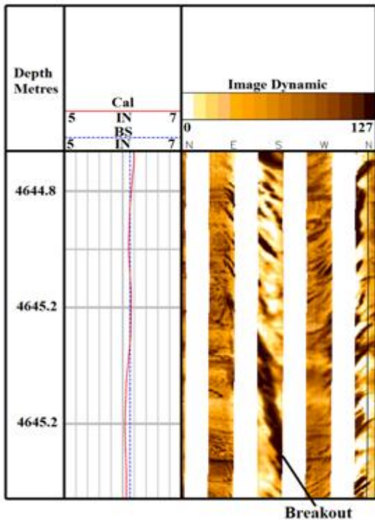
Figure 8) One of the recognized breakouts in image log of the borehole. The tracks are depth, Bit Size – Caliper and dynamic image log left to right respectively. In middle track Bit Size and Caliper logs are coincident approximately but in lower part of the track Caliper is less than Bit Size that causes mud cake creation in this part.
