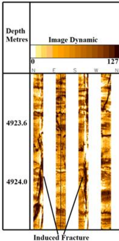
Figure 9) Induced fracture in image log.
